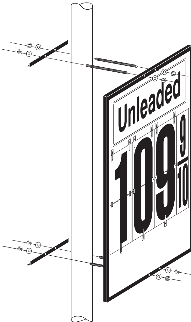
SINGLE SIGN POLE MOUNT
